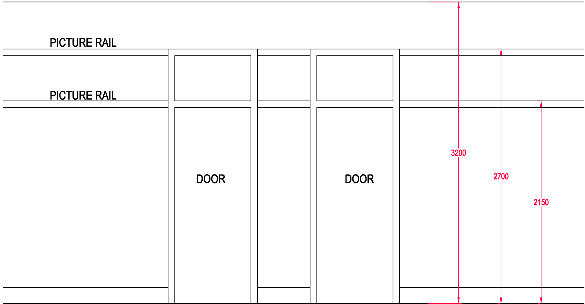
TYPICAL WALL ELEVATION
