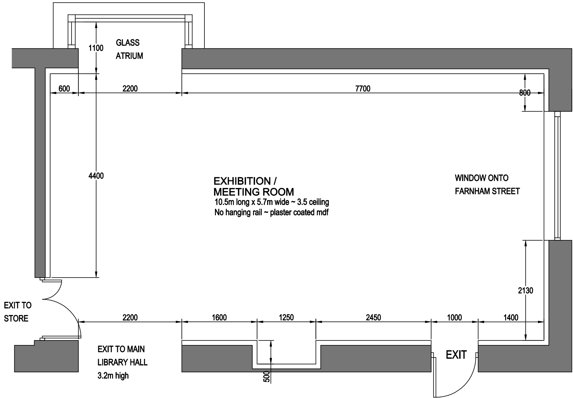
JOHNSTON CENTRAL LIBRARY & FARNHAM CENTRE Ground Floor Plan
